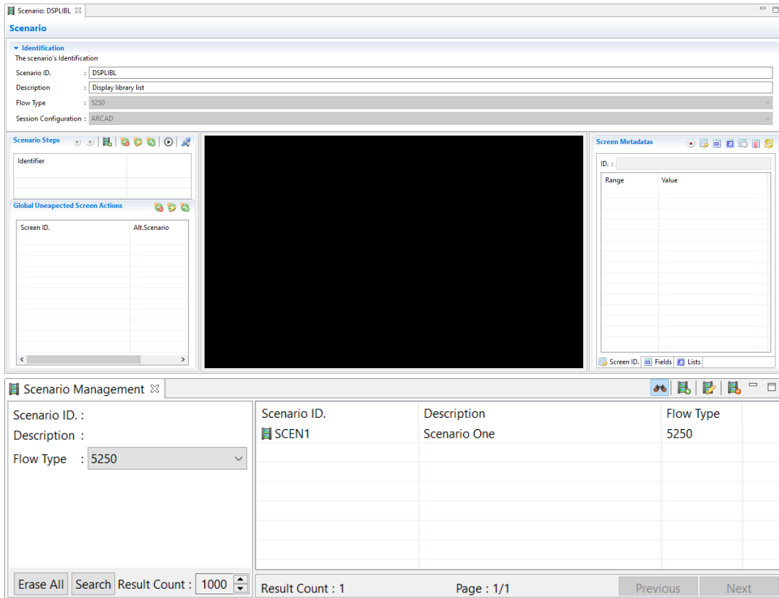
Figure 38: The Scenario editor
